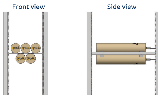
19" Rails Hor. for 3+2 x CAV125mm P. no. 210003059 (Note cavities not included)
