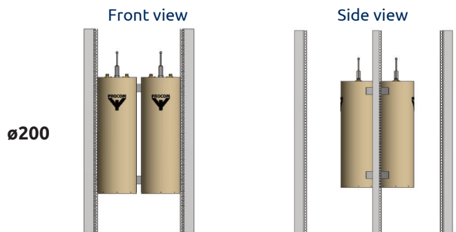
19" Rails Ver. for 2+2 x CAV200mm P. no. 210003068 (Note cavities not included)
