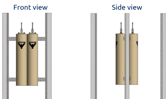
19" Rails Ver. for 2+2 x CAV125mm P. no. 210003056 (Note cavities not included)
