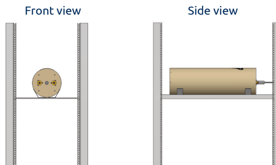
19" Rails Hor. for 1 x CAV200mm P. no. 210003063 (Note cavities not included)
