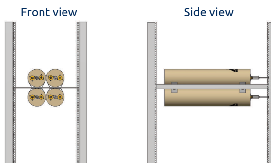
19" Rails Hor. for 2+2 x CAV125mm P. no. 210003057 (Note cavities not included)
