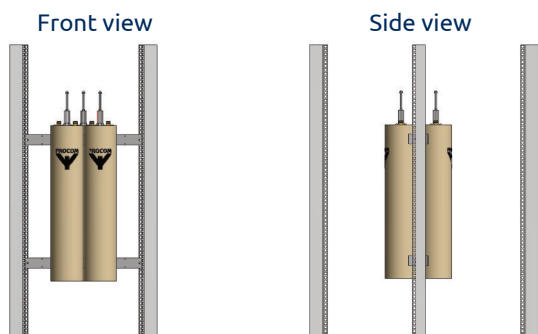
19" Rails Ver. for 2+1 x CAV125mm P. no. 210003054 (Note cavities not included)
