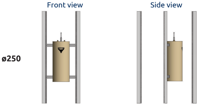
19" Rails Ver. for 1 x CAV250mm P. no. 210003070 (Note cavities not included)
