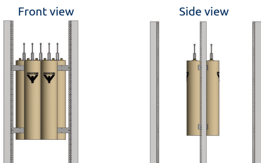
19" Rails Ver. for 3+2 x CAV125mm P. no. 210003058 (Note cavities not included)
