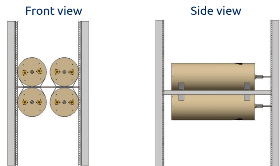
19" Rails Hor. for 2+2 x CAV200mm P. no. 210003069 (Note cavities not included)
