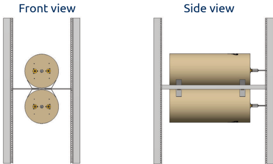
19" Rails Hor. for 1+1 x CAV250mm P. no. 210003074 (Note cavities not included)
