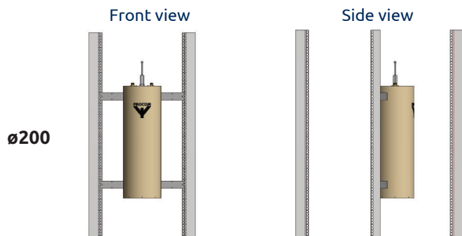
19" Rails Ver. for 1 x CAV200mm P. no. 210003062 (Note cavities not included)
