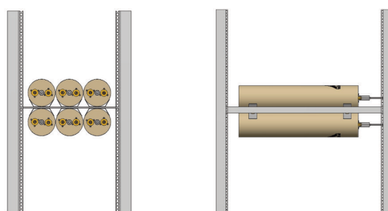
19" Rails Hor. for 3+3 x CAV125mm P. no. 210003061 (Note cavities not included)
