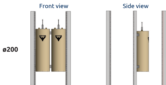
19" Rails Ver. for 2 x CAV200mm P. no. 210003064 (Note cavities not included)
