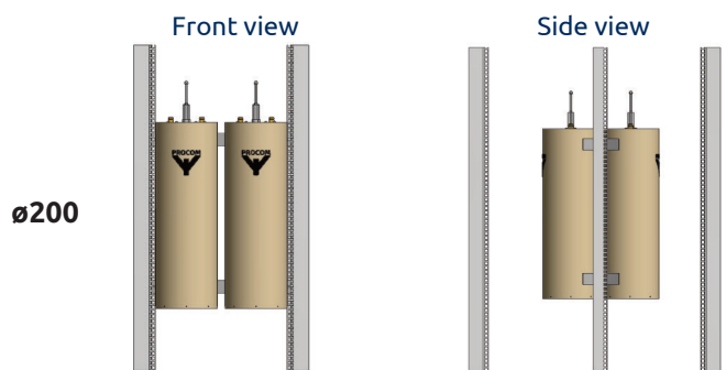
19" Rails Ver. for 2+1 x CAV200mm P. no. 210003066 (Note cavities not included)
