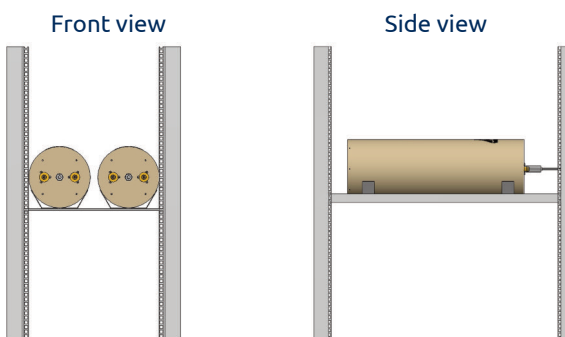
19" Rails Hor. for 2 x CAV200mm P. no. 210003065 (Note cavities not included)
