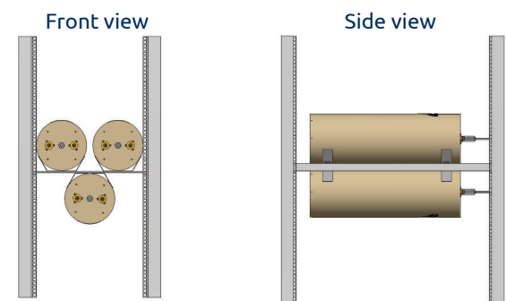
19" Rails Hor. for 2+1 x CAV200mm P. no. 210003067 (Note cavities not included)
