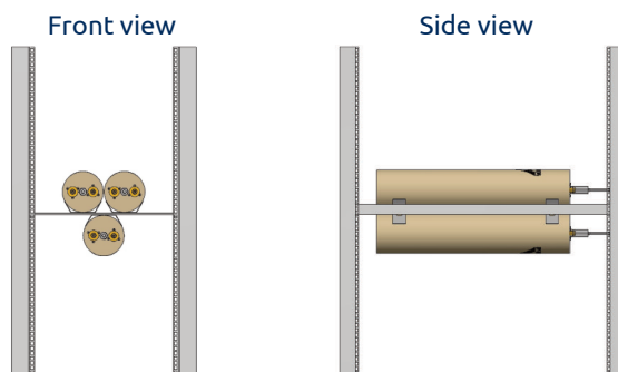
19" Rails Hor. for 2+1 x CAV125mm P. no. 210003055 (Note cavities not included)
