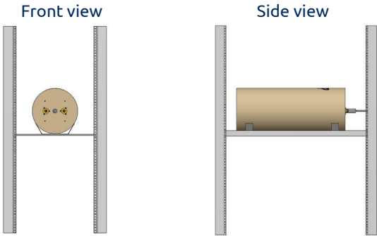
19" Rails Hor. for 1 x CAV250mm P. no. 210003071 (Note cavities not included)
